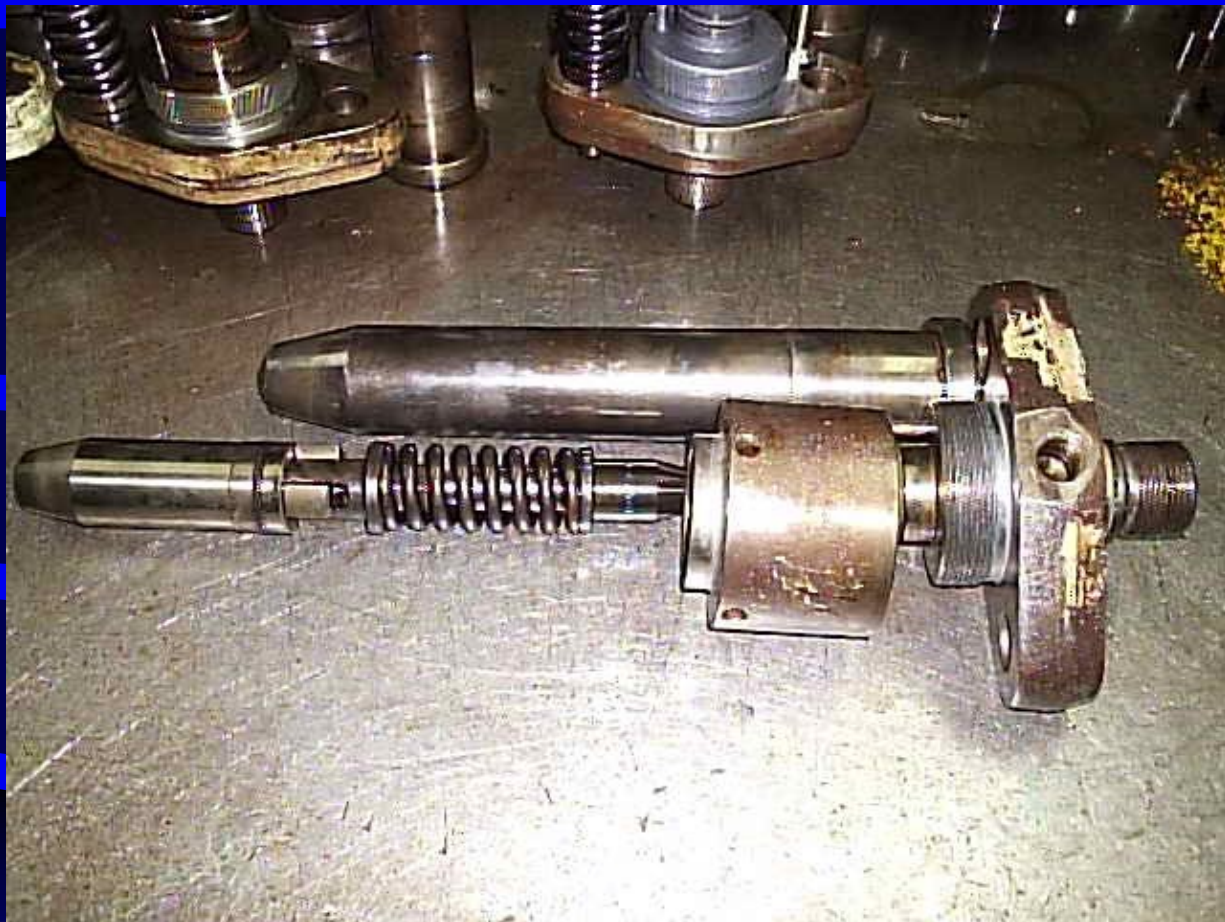
INJETOR DO MOTOR MKOTOR MAN – B&W 5 L 50 MC
